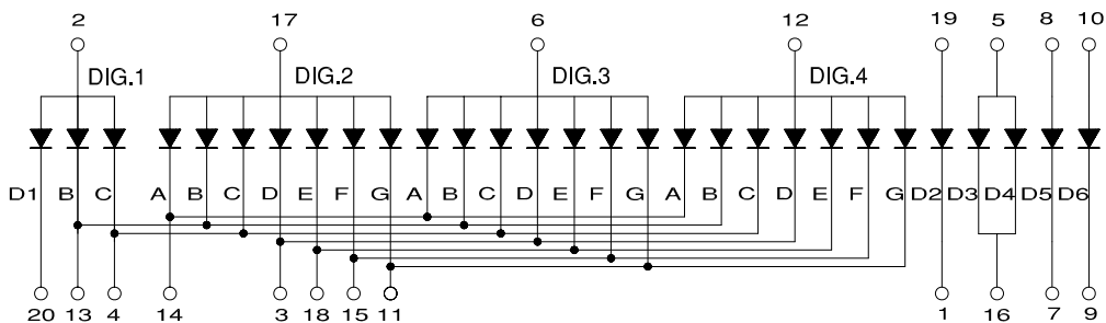
SCD-337 (Anode Common)
